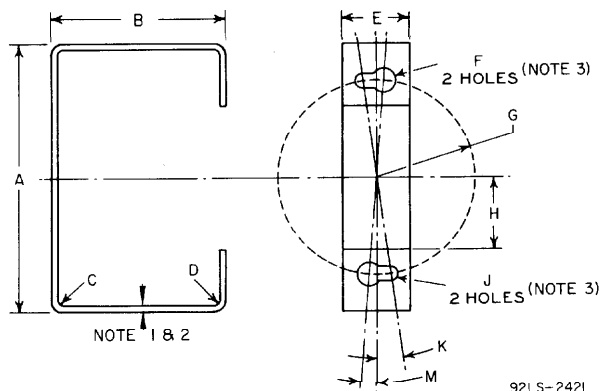
Figure 1 - Tube Extractor - Suggested Design
