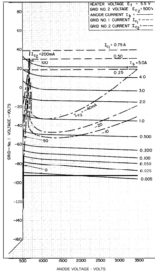
Figure 3 - Typical Constant Current Characteristics ( E_{c2} = 500 \text{ V} )
