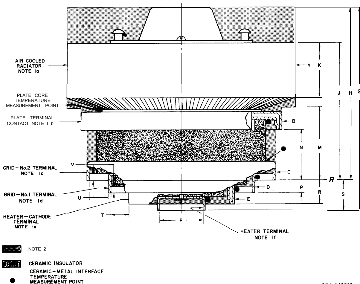
Figure 5 - Dimensional Outline
