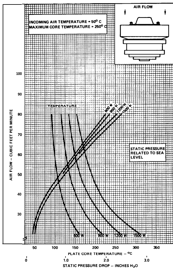
Figure 7 - Typical Cooling Characteristics
